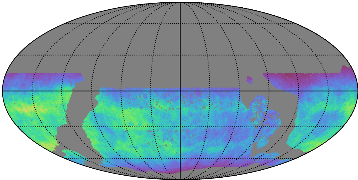
extra_ss_neo7_v3.4_10yrs WFD u band: Normalized Teff
