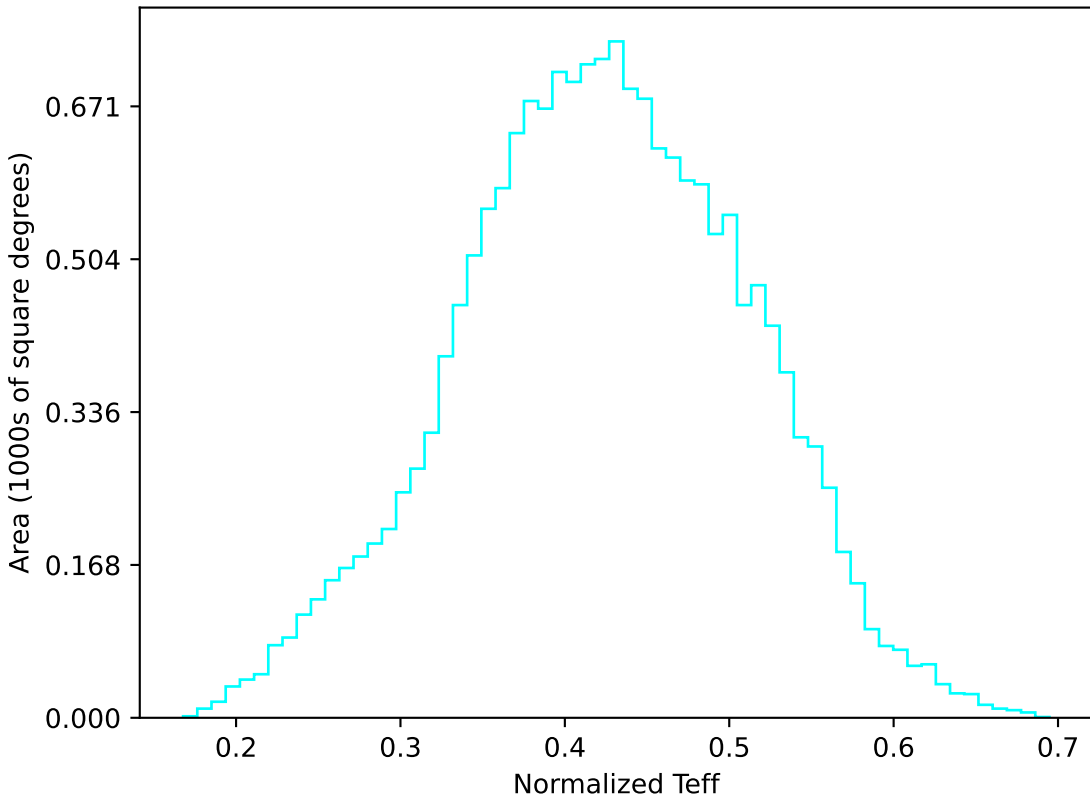
extra_ss_neo7_v3.4_10yrs WFD u band: Normalized Teff
