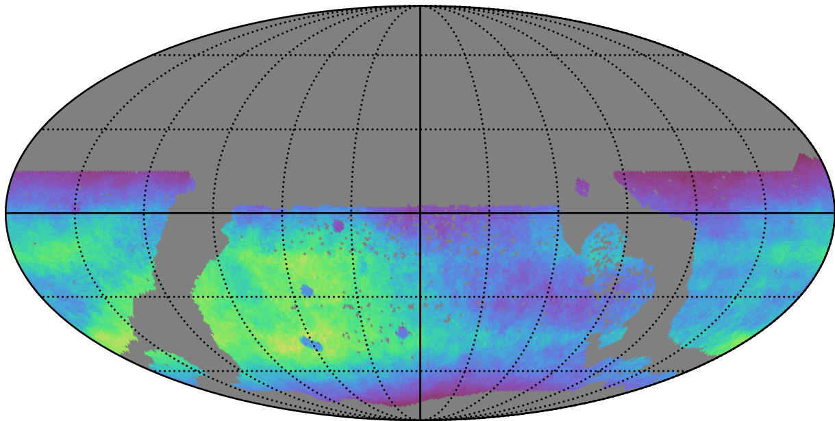
extra_ss_neo7_v3.4_10yrs WFD r band: Normalized Teff
