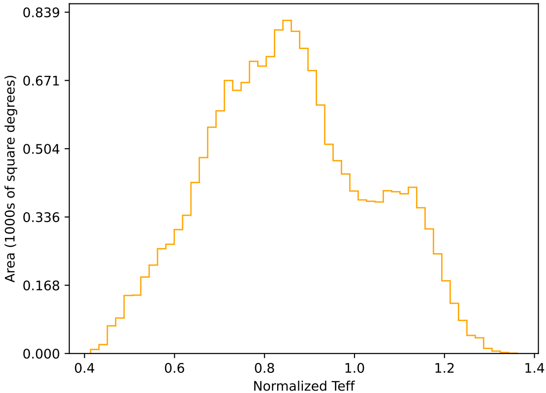
extra_ss_neo7_v3.4_10yrs WFD r band: Normalized Teff
