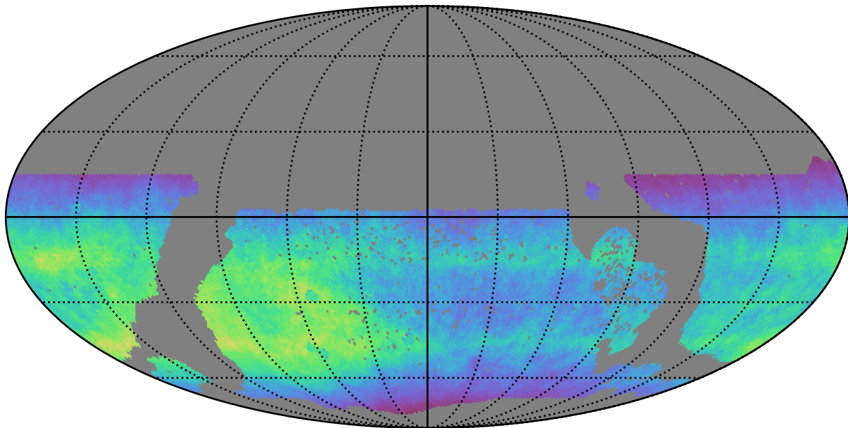
extra_ss_neo7_v3.4_10yrs WFD i band: Normalized Teff
