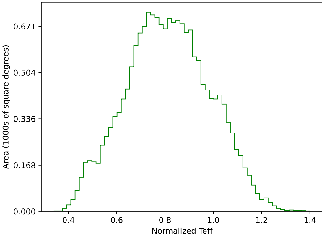
extra_ss_neo7_v3.4_10yrs WFD g band: Normalized Teff
