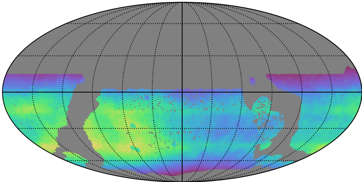
extra_ss_neo7_v3.4_10yrs WFD all bands: Normalized Teff
