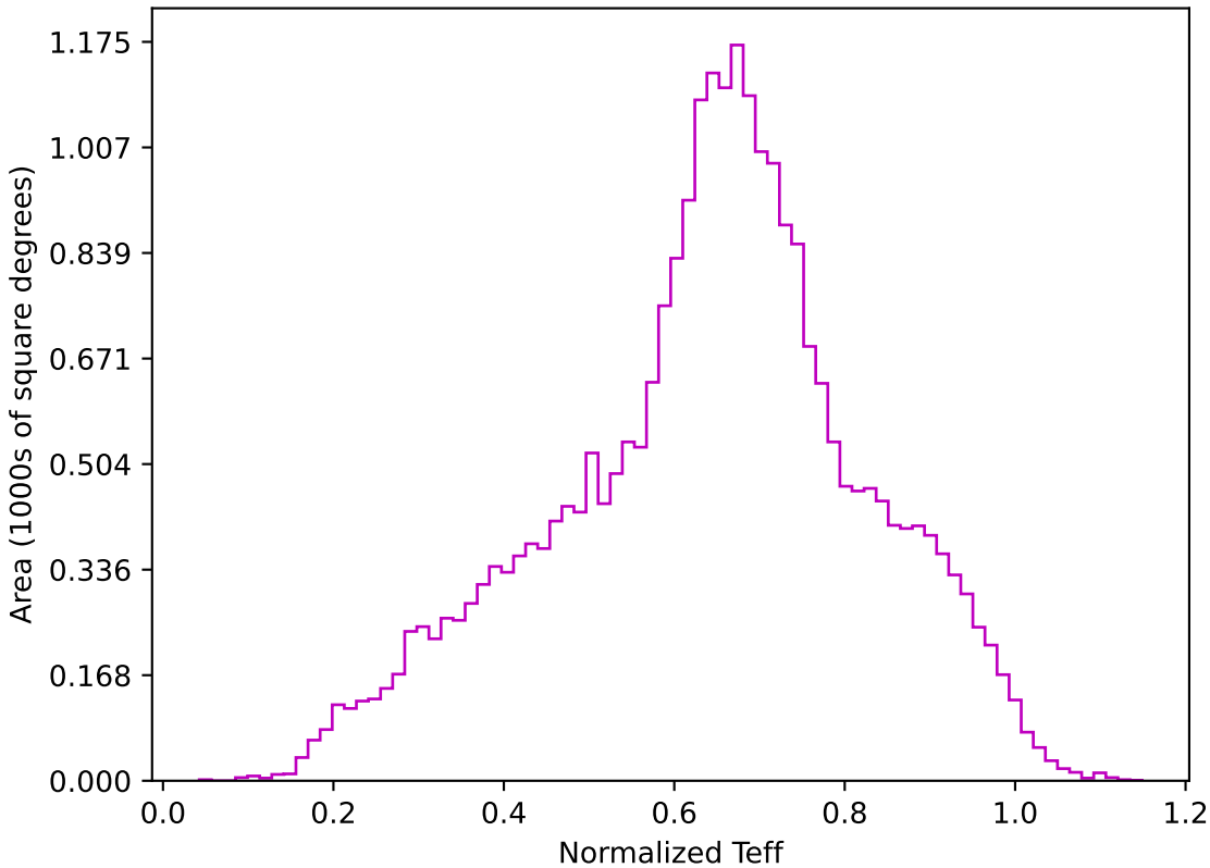
extra_ss_neo7_v3.4_10yrs All sky z band: Normalized Teff
