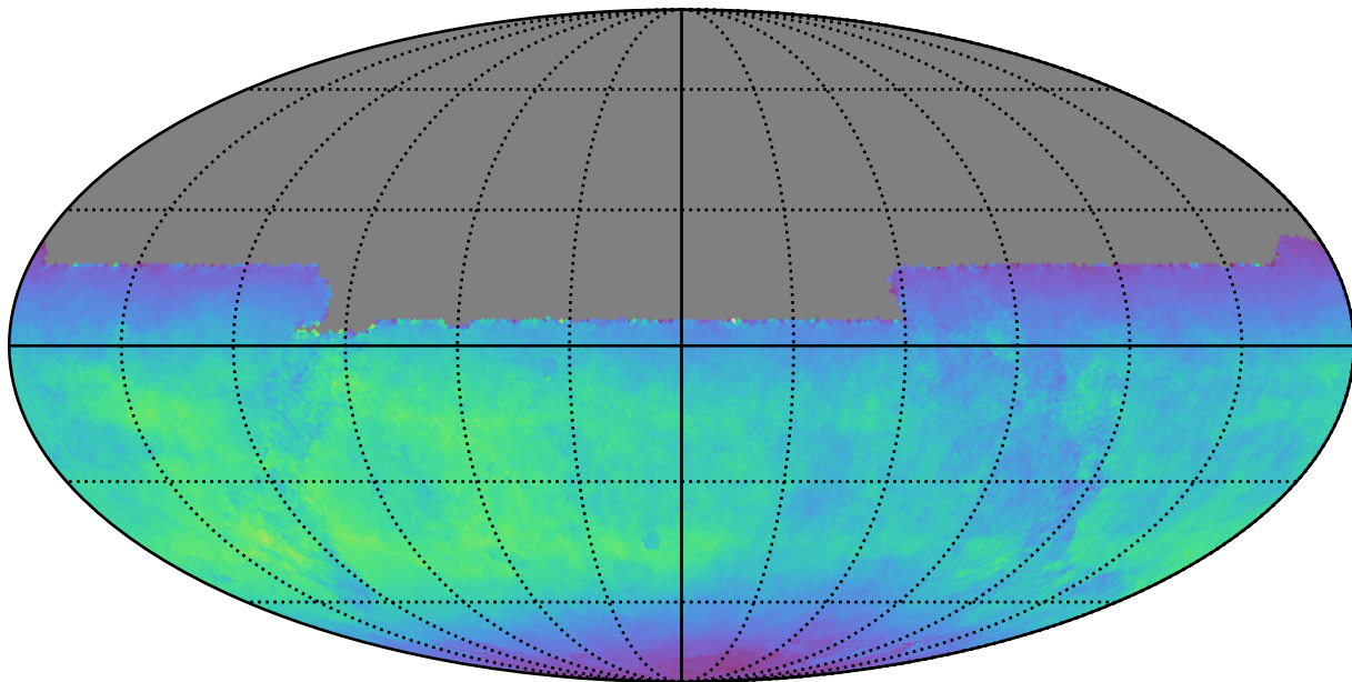
extra_ss_neo7_v3.4_10yrs All sky y band: Normalized Teff
