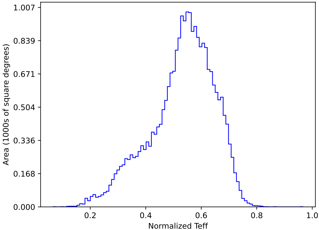
extra_ss_neo7_v3.4_10yrs All sky y band: Normalized Teff
