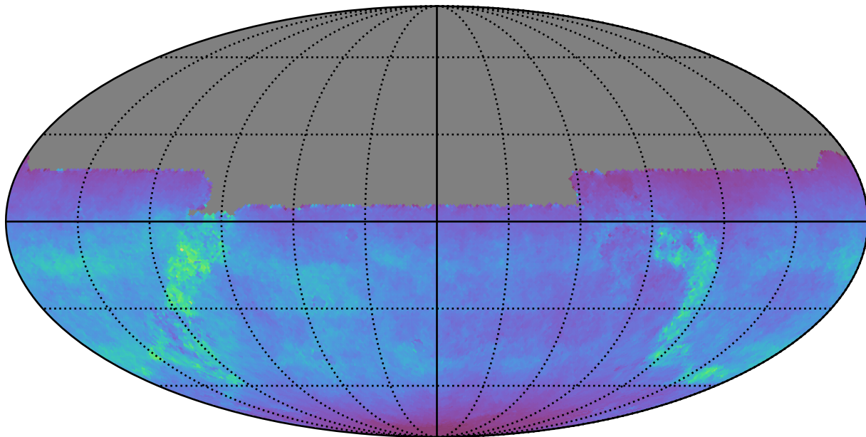
extra_ss_neo7_v3.4_10yrs All sky u band: Normalized Teff
