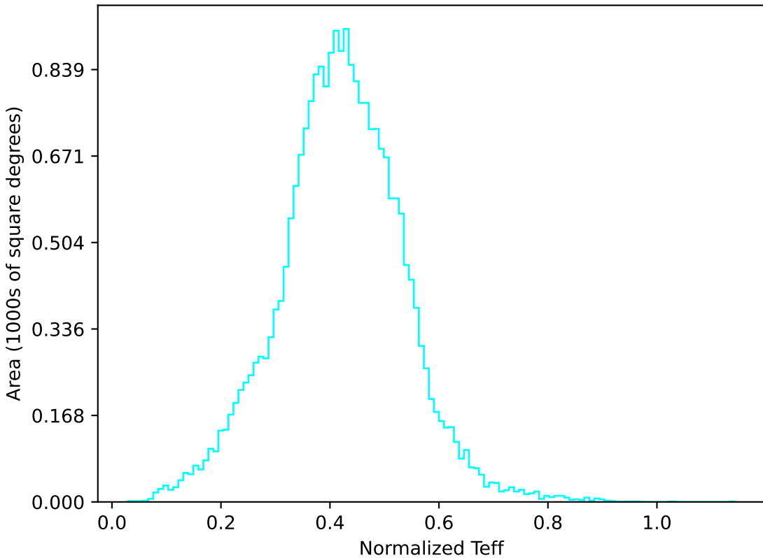
extra_ss_neo7_v3.4_10yrs All sky u band: Normalized Teff
