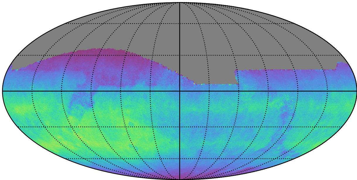
extra_ss_neo7_v3.4_10yrs All sky i band: Normalized Teff
