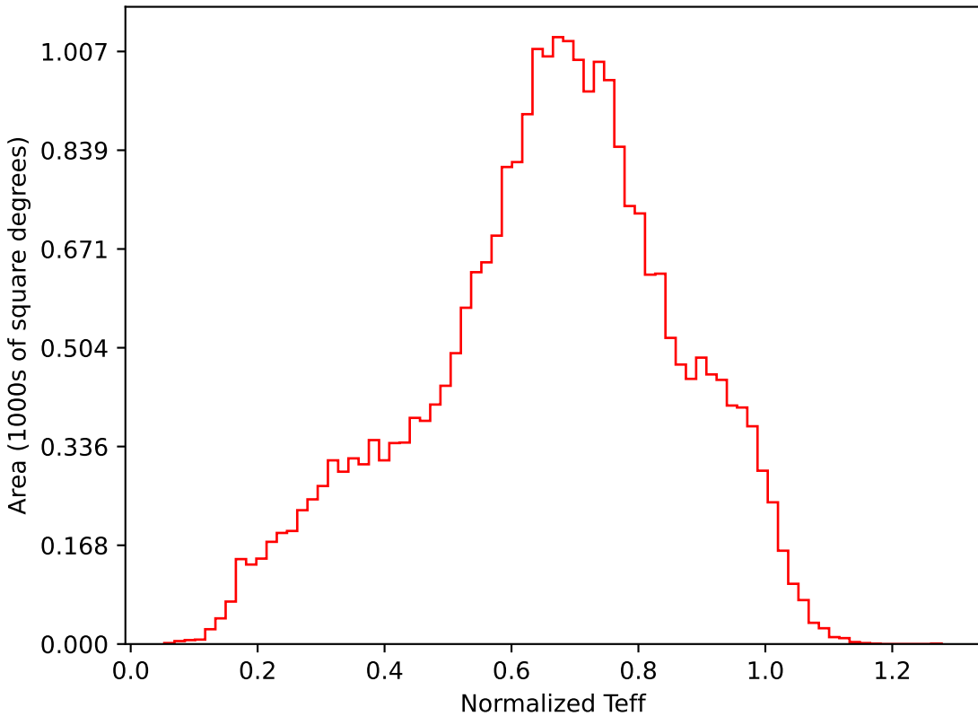
extra_ss_neo7_v3.4_10yrs All sky i band: Normalized Teff
