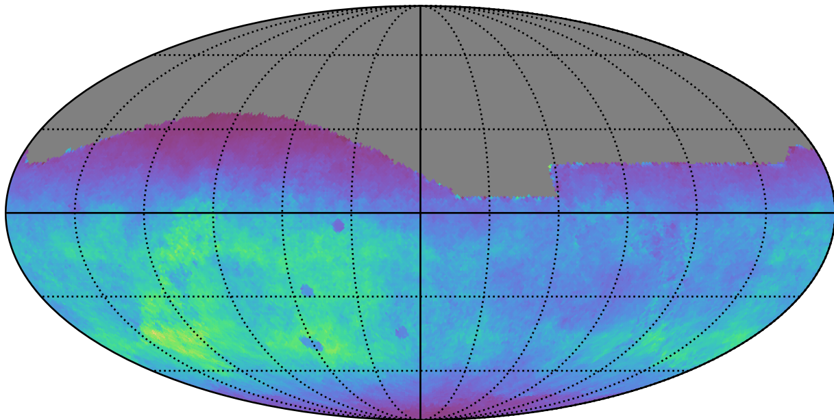
extra_ss_neo7_v3.4_10yrs All sky g band: Normalized Teff
