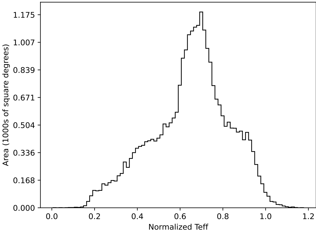
extra_ss_neo7_v3.4_10yrs All sky all bands: Normalized Teff
