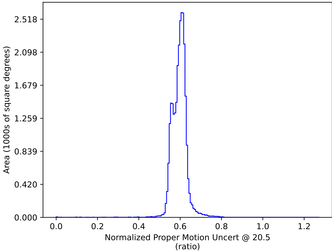
extra_ss_neo7_v3.4_10yrs All sky: Normalized Proper Motion Uncert @ 20.5
