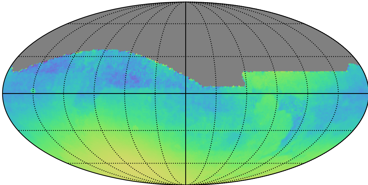
extra_ss_neo7_v3.4_10yrs All sky: Normalized Parallax Uncert @ 24.0
