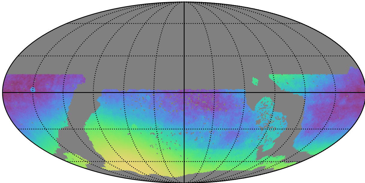
extra_ss_neo7_v3.4_10yrs WFD: Normalized Parallax Uncert @ 22.4
