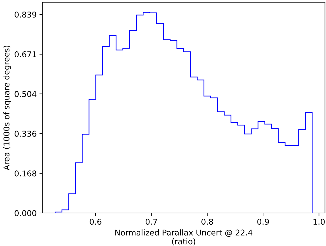
extra_ss_neo7_v3.4_10yrs WFD: Normalized Parallax Uncert @ 22.4
