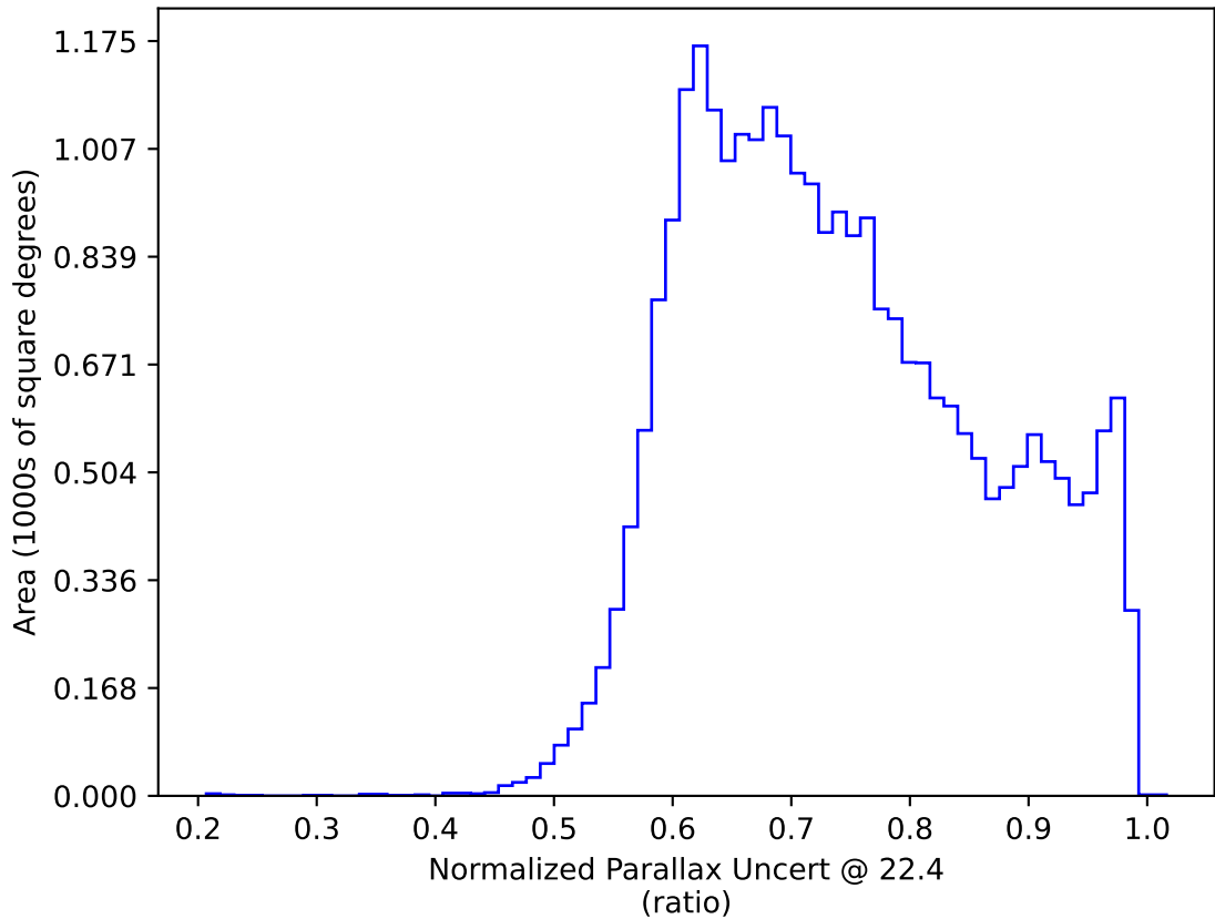
extra_ss_neo7_v3.4_10yrs All sky: Normalized Parallax Uncert @ 22.4
