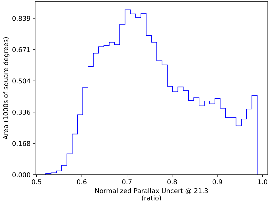
extra_ss_neo7_v3.4_10yrs WFD y band only: Normalized Parallax Uncert @ 21.3
