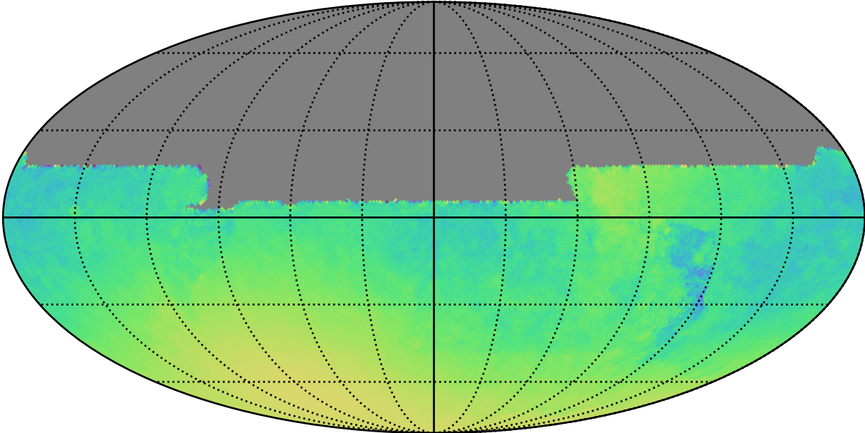
extra_ss_neo7_v3.4_10yrs All sky y band only: Normalized Parallax Uncert @ 21.3
