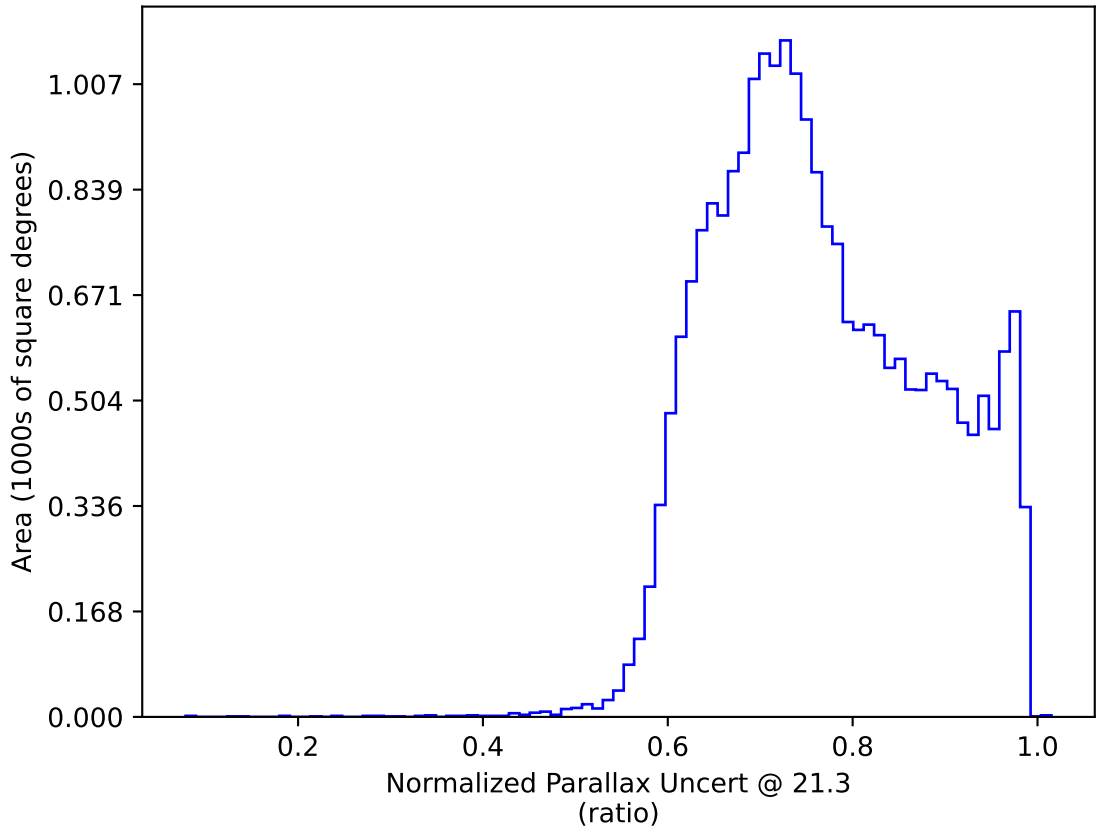
extra_ss_neo7_v3.4_10yrs All sky y band only: Normalized Parallax Uncert @ 21.3
