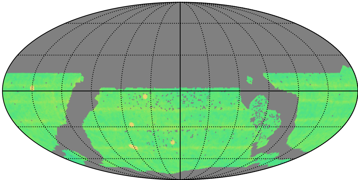
extra_ss_neo7_v3.4_10yrs WFD all bands: N Unique Nights
