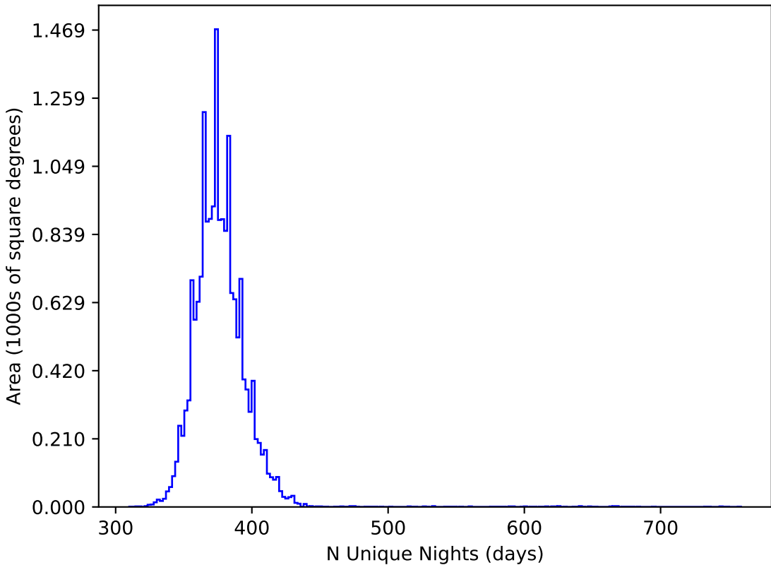
extra_ss_neo7_v3.4_10yrs WFD all bands: N Unique Nights
