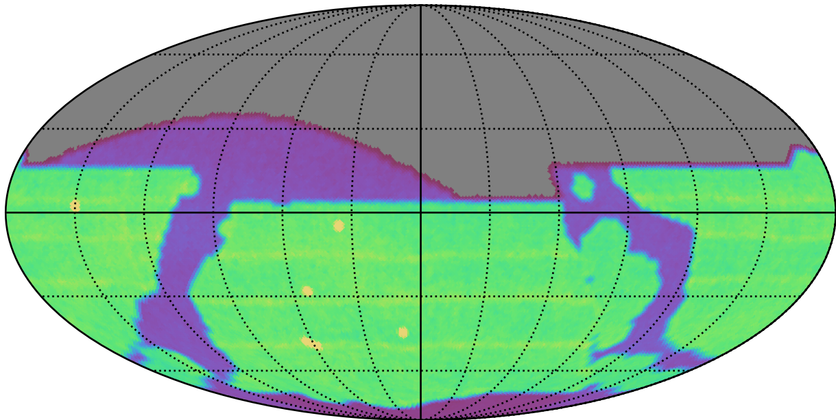
extra_ss_neo7_v3.4_10yrs All sky all bands: N Unique Nights
