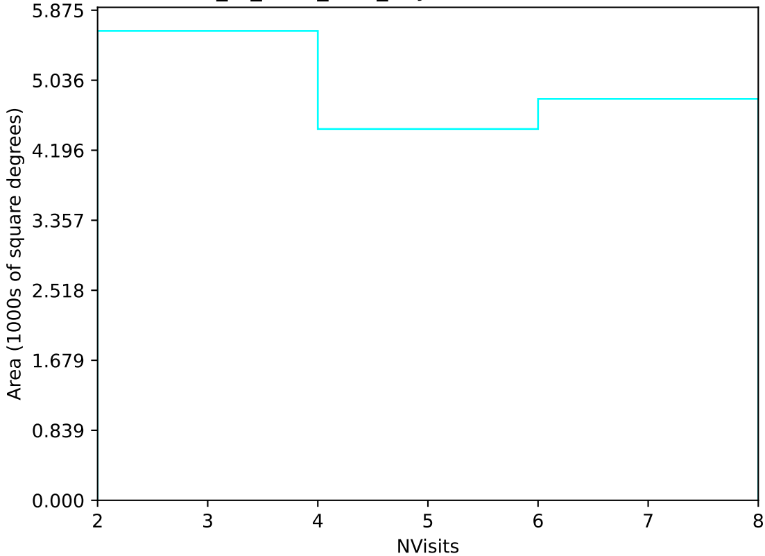
extra_ss_neo7_v3.4_10yrs Yr 3-4 u band: NVisits
