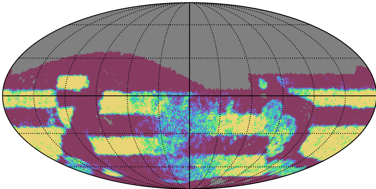
extra_ss_neo7_v3.4_10yrs Yr 3-4 r band: NVisits
