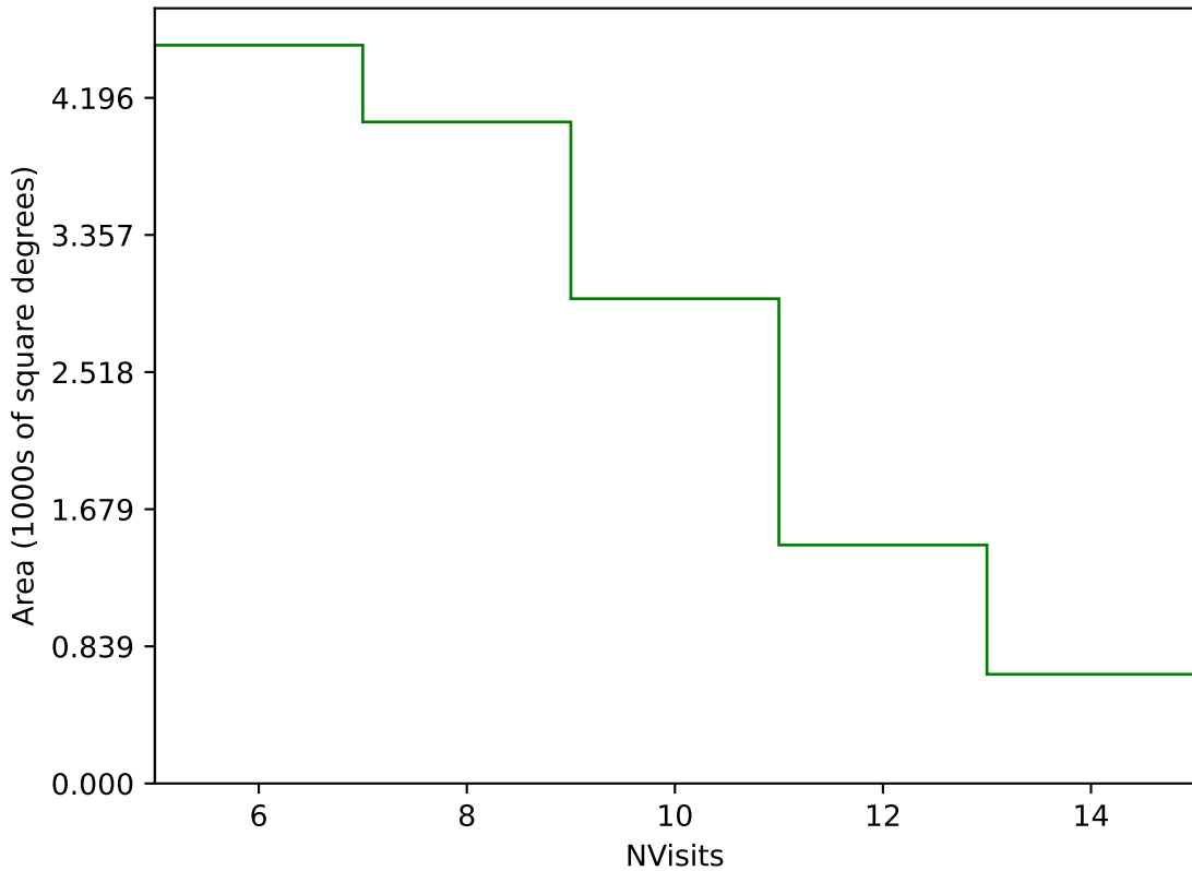
extra_ss_neo7_v3.4_10yrs Yr 3-4 g band: NVisits
