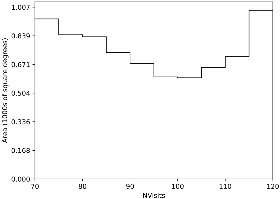
extra_ss_neo7_v3.4_10yrs Yr 3-4 all bands: NVisits
