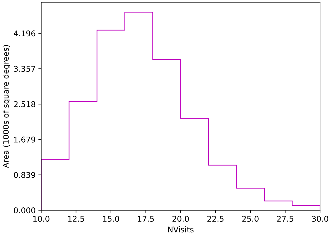
extra_ss_neo7_v3.4_10yrs Yr 1 z band: NVisits
