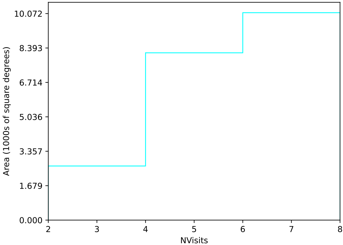
extra_ss_neo7_v3.4_10yrs Yr 1 u band: NVisits
