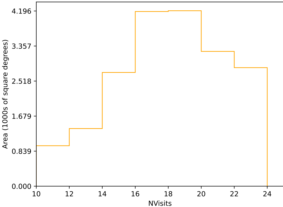
extra_ss_neo7_v3.4_10yrs Yr 1 r band: NVisits
