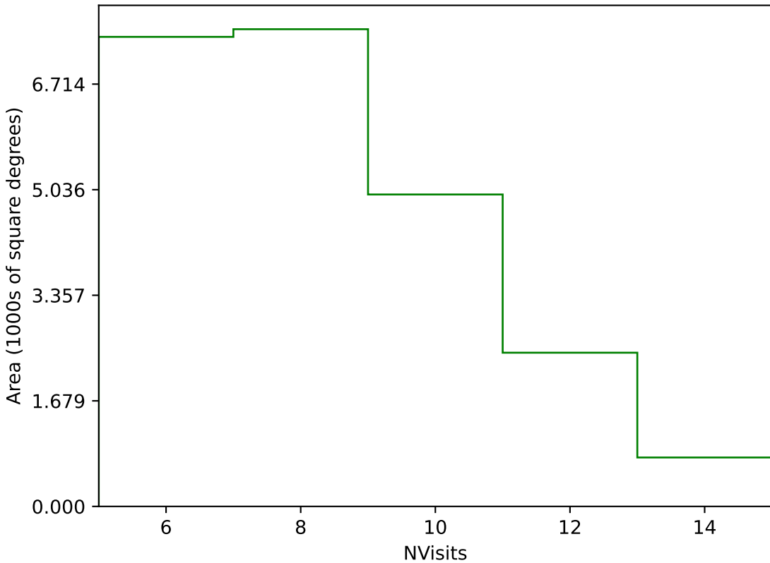
extra_ss_neo7_v3.4_10yrs Yr 1 g band: NVisits
