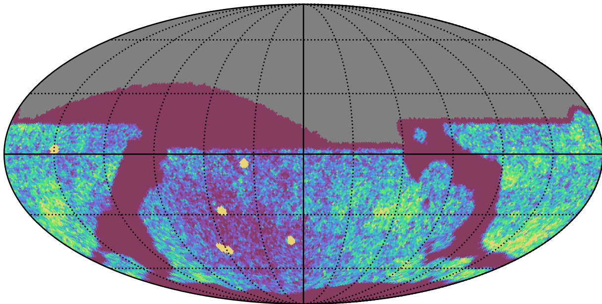
extra_ss_neo7_v3.4_10yrs Yr 1 all bands: NVisits
