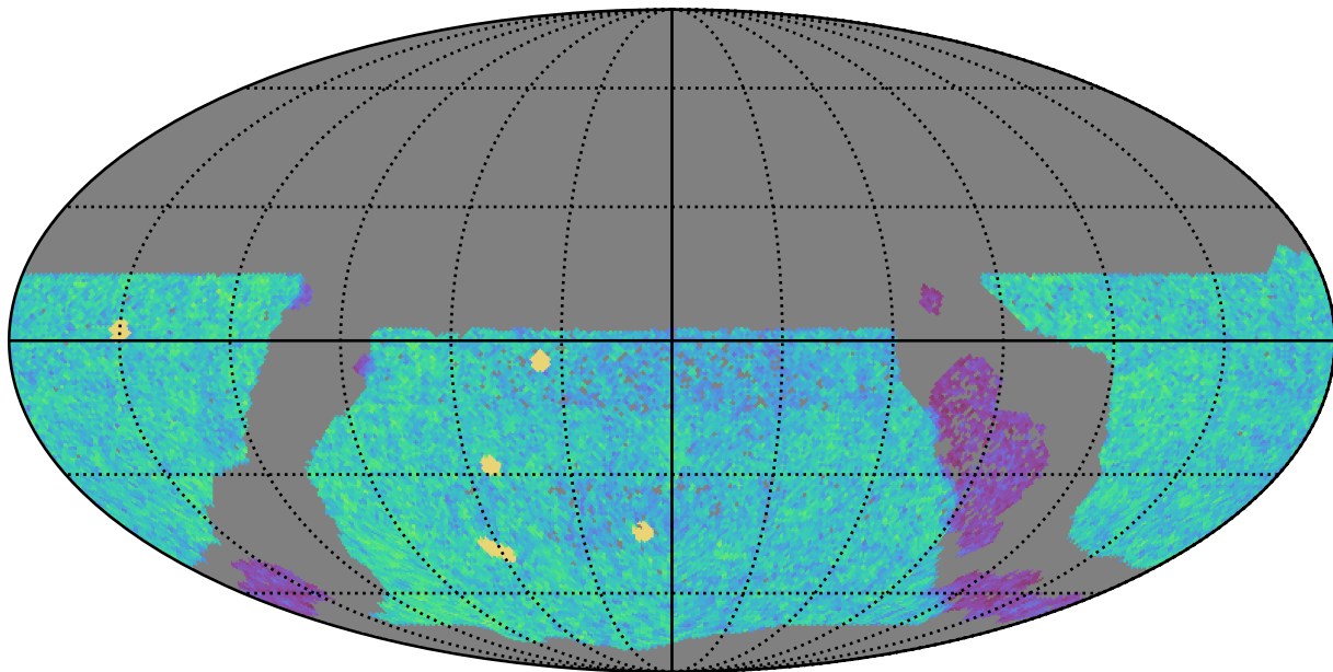
extra_ss_neo7_v3.4_10yrs WFD u band: NVisits
