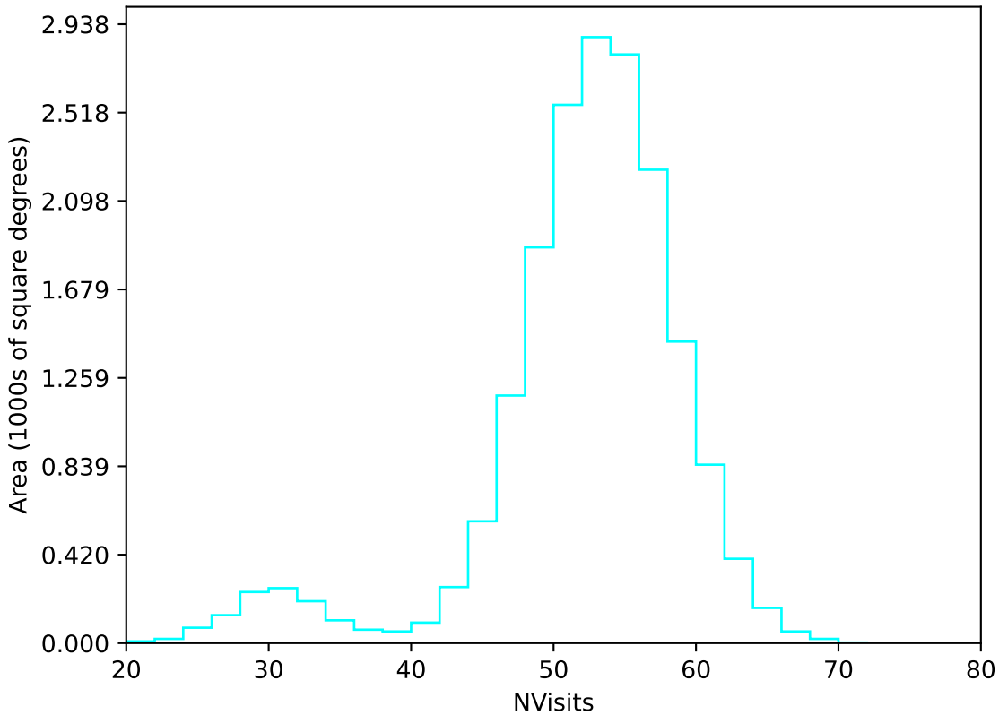
extra_ss_neo7_v3.4_10yrs WFD u band: NVisits
