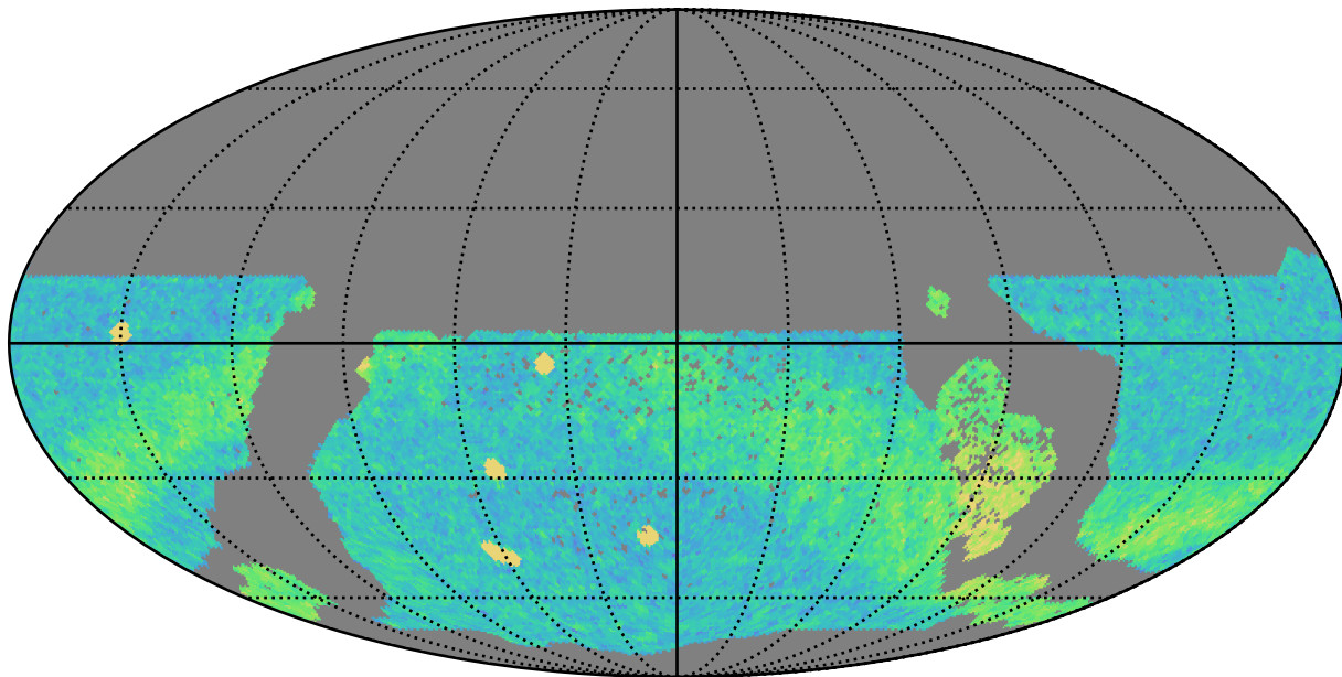
extra_ss_neo7_v3.4_10yrs WFD r band: NVisits
