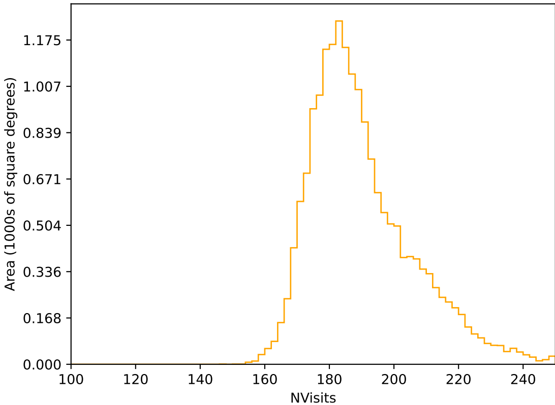
extra_ss_neo7_v3.4_10yrs WFD r band: NVisits
