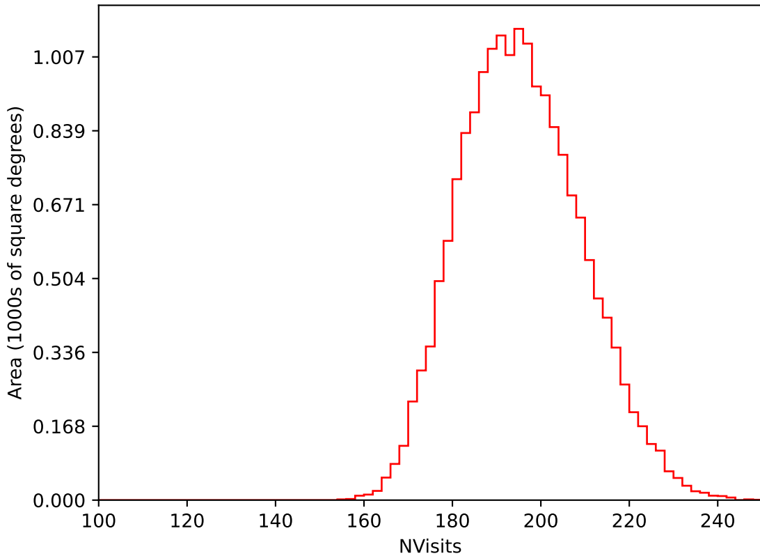
extra_ss_neo7_v3.4_10yrs WFD i band: NVisits
