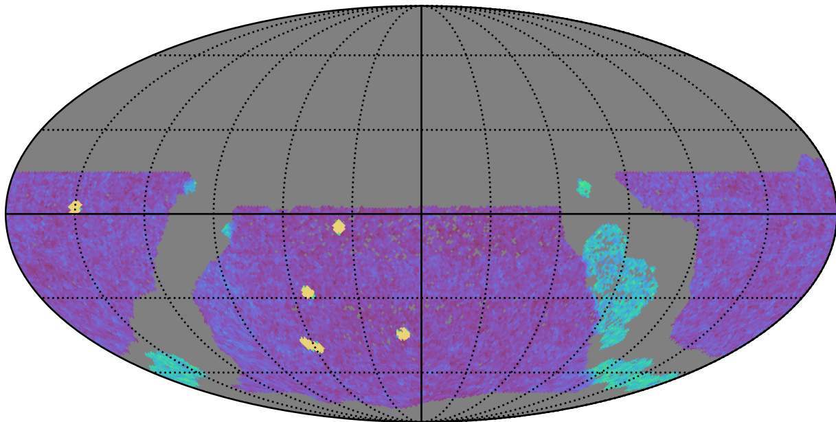
extra_ss_neo7_v3.4_10yrs WFD g band: NVisits
