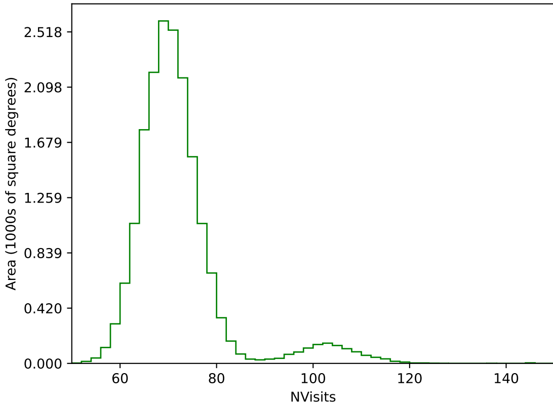
extra_ss_neo7_v3.4_10yrs WFD g band: NVisits
