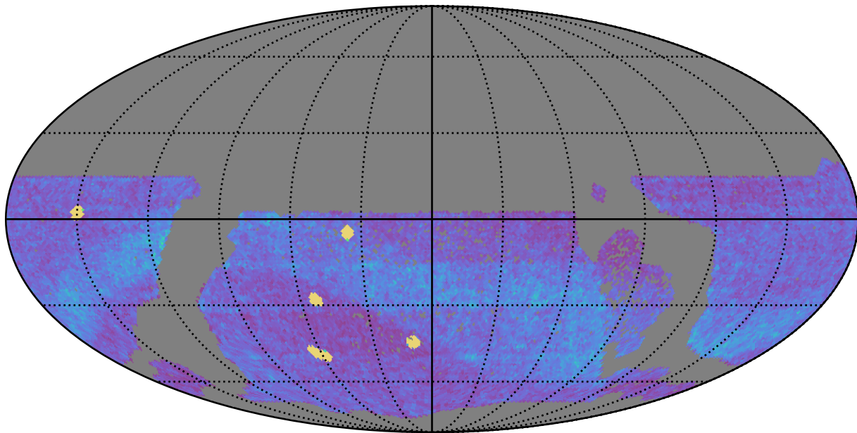
extra_ss_neo7_v3.4_10yrs WFD all bands: NVisits
