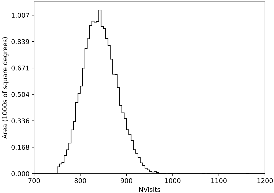
extra_ss_neo7_v3.4_10yrs WFD all bands: NVisits
