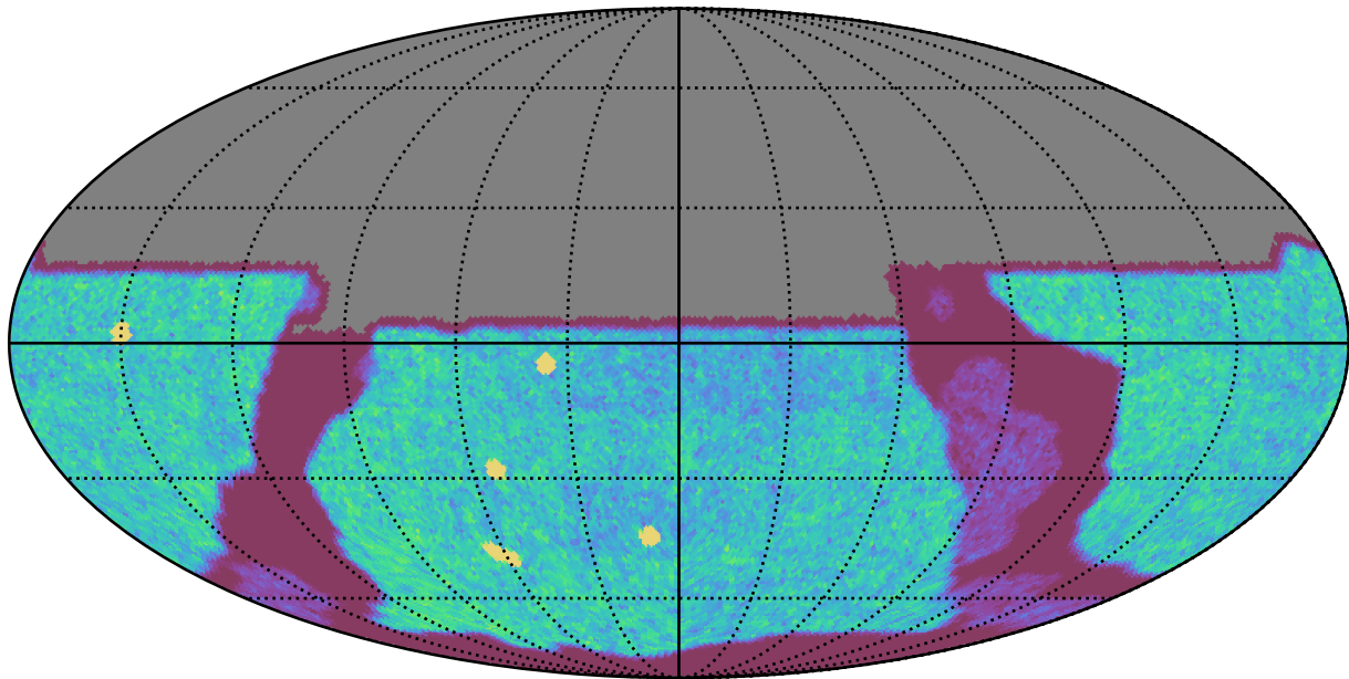
extra_ss_neo7_v3.4_10yrs All sky u band: NVisits
