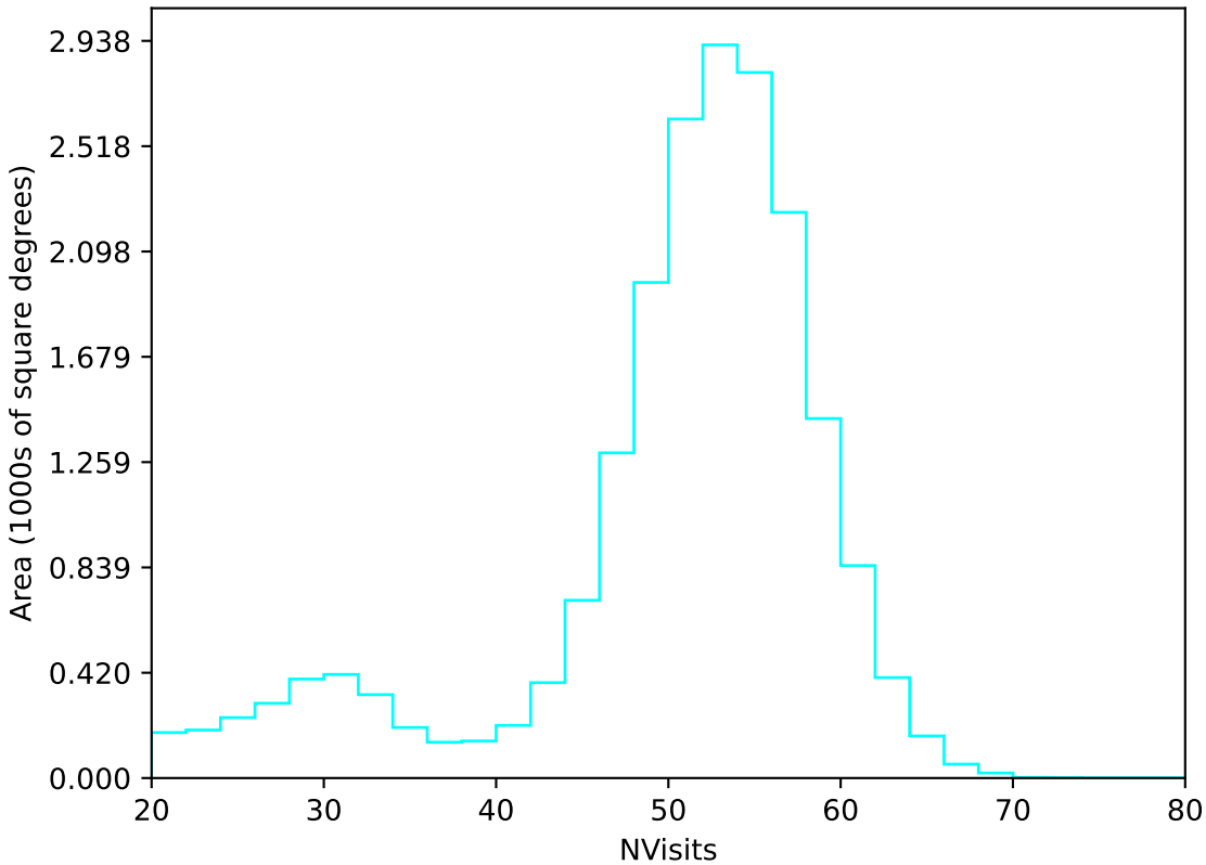
extra_ss_neo7_v3.4_10yrs All sky u band: NVisits
