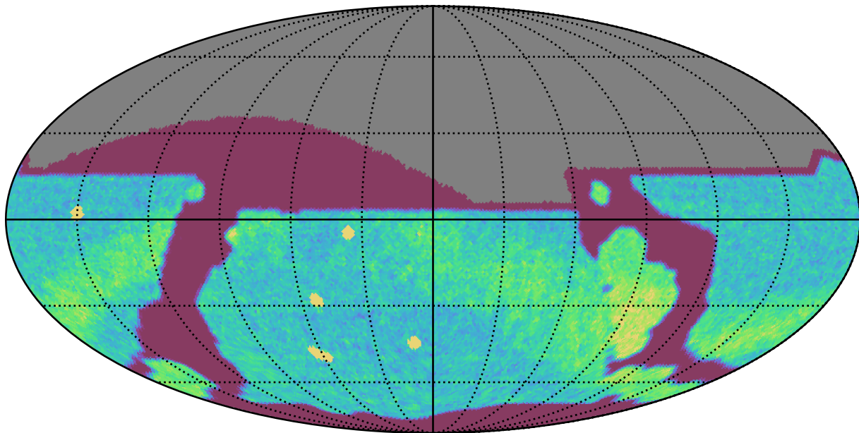
extra_ss_neo7_v3.4_10yrs All sky r band: NVisits
