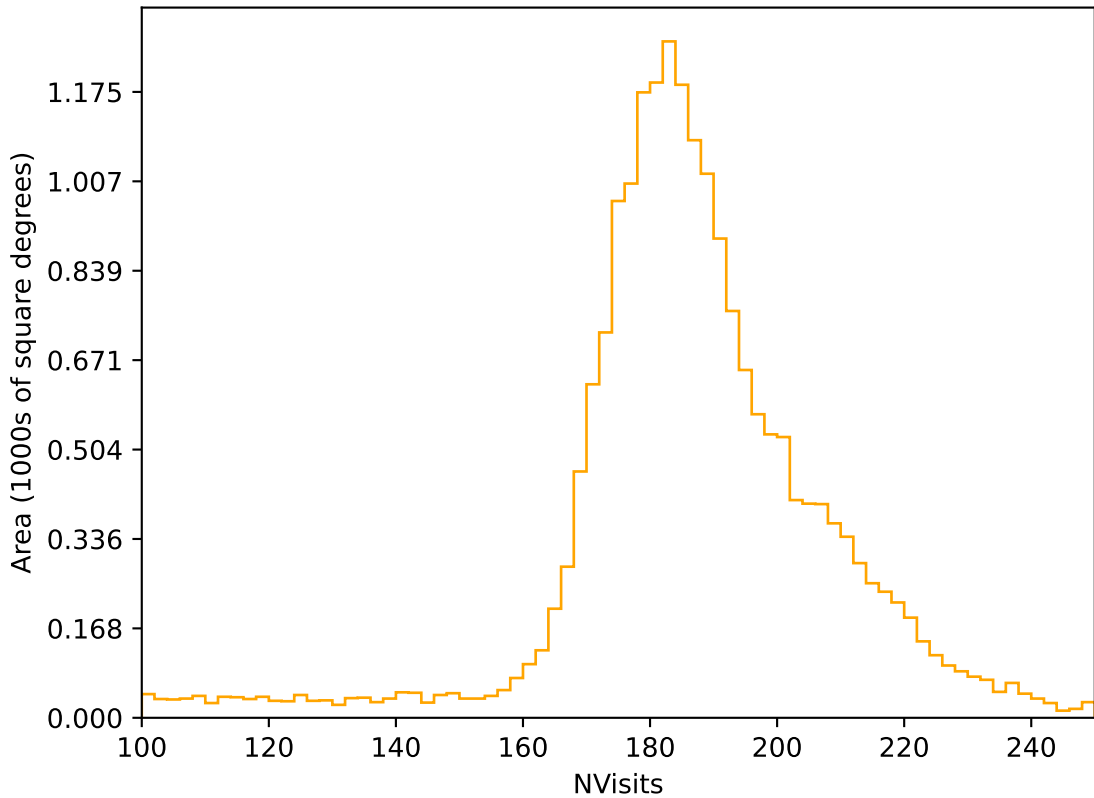
extra_ss_neo7_v3.4_10yrs All sky r band: NVisits
