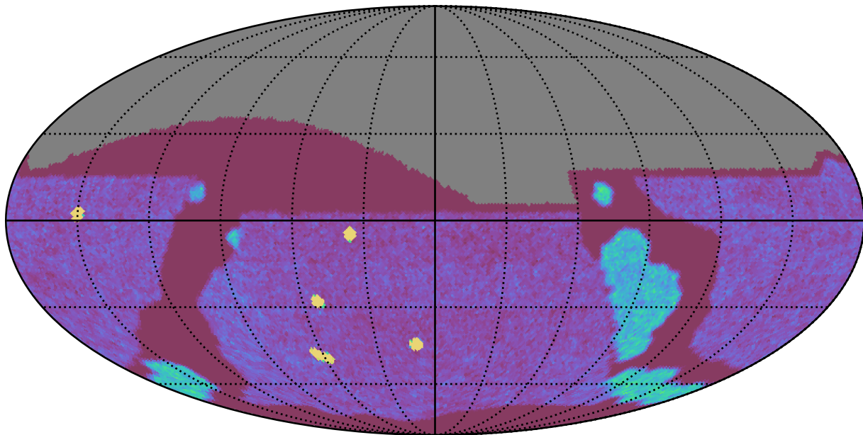
extra_ss_neo7_v3.4_10yrs All sky g band: NVisits
